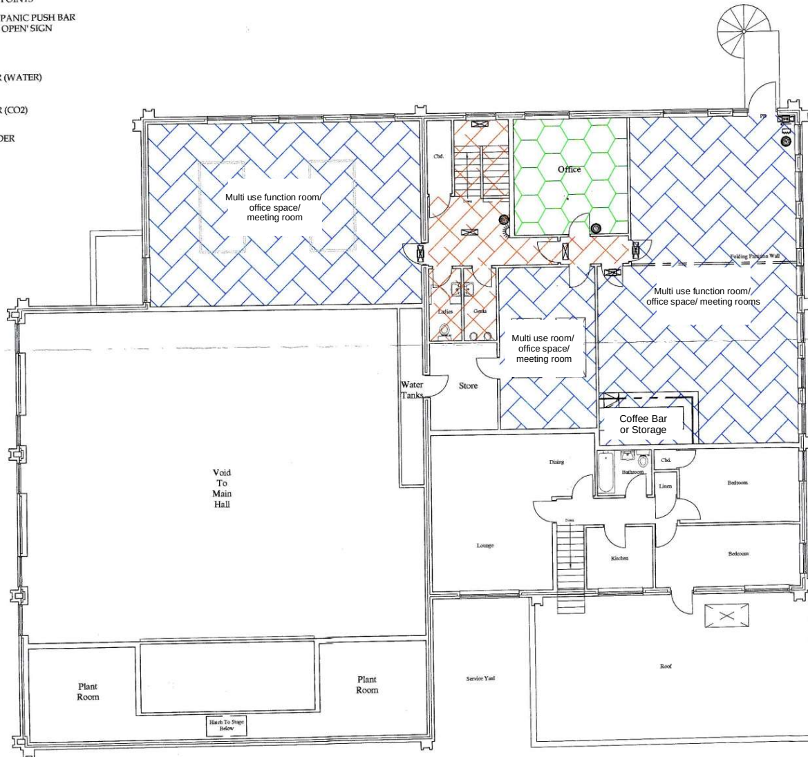
First Floor - 1:100
