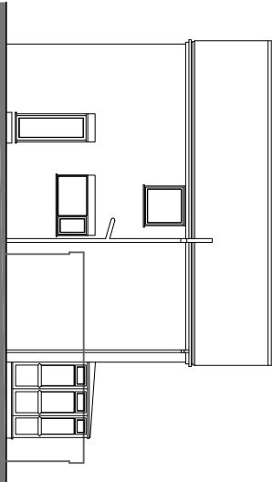
EXISTING SIDE ELEVATION 1:100@A1
