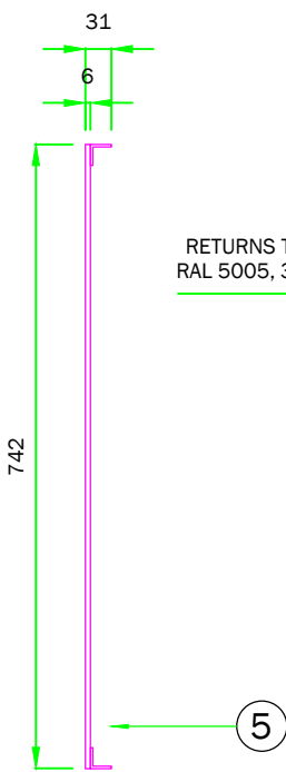
Base Plate: End Elevation scale 1:10
