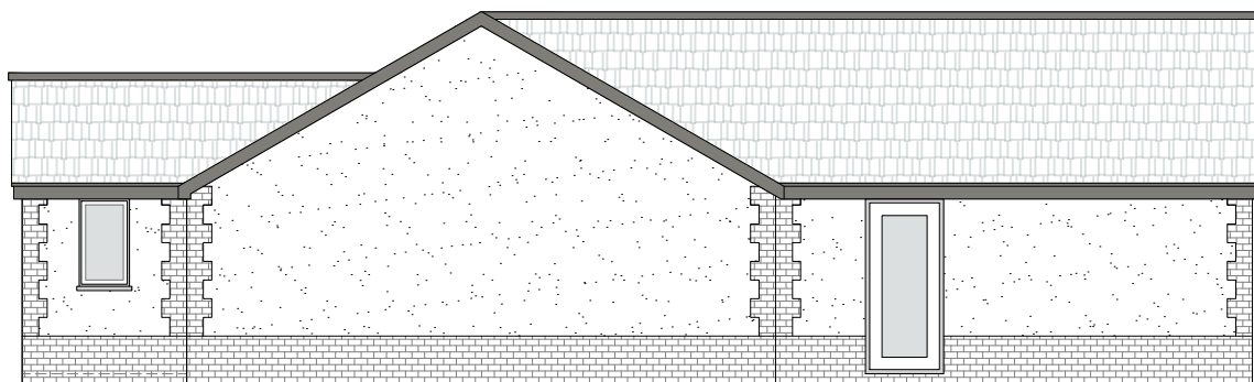
Proposed North Side Elevation - 1:100
