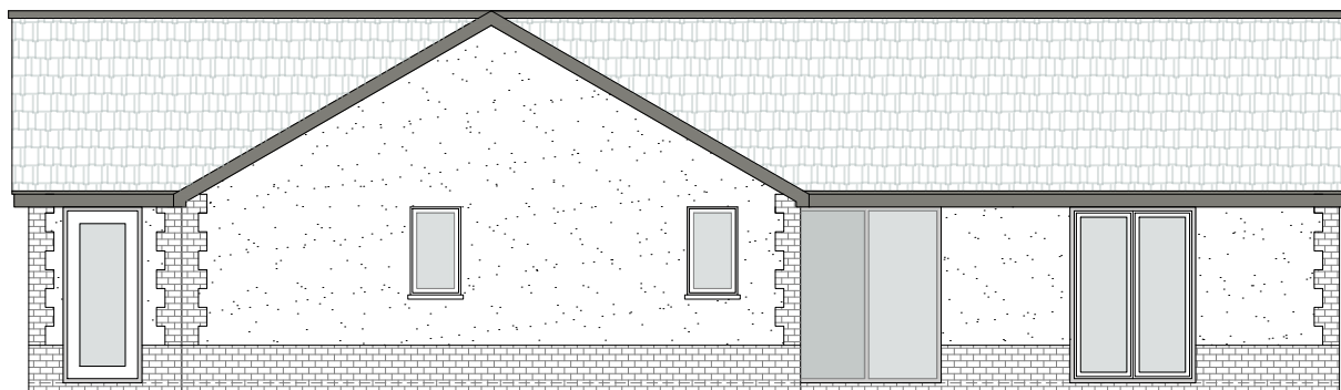
Proposed Rear Elevation - 1:100
