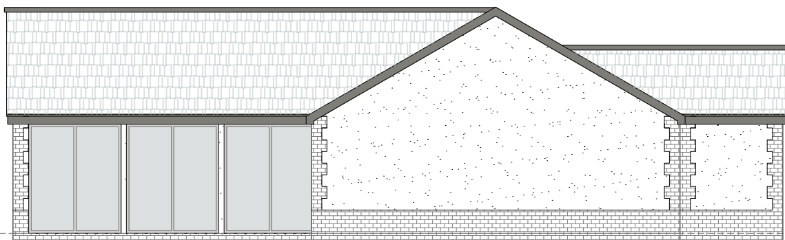
Proposed South Side Elevation - 1:100
