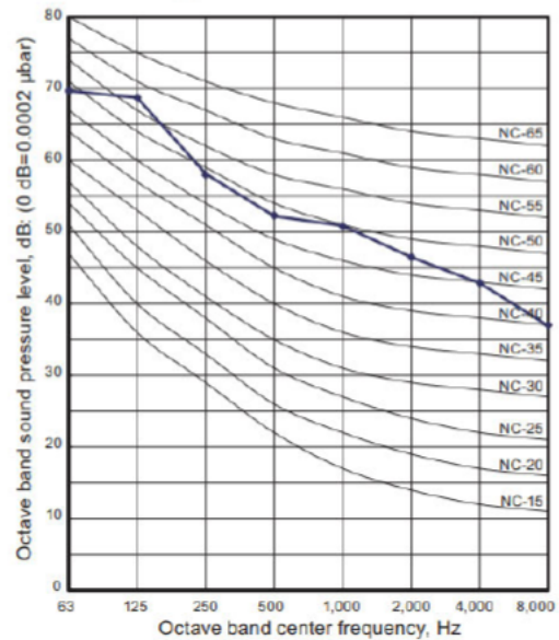
Figure 6.3.2 – Noise Data – Proposed Condenser – 109 Winchester Rd.
