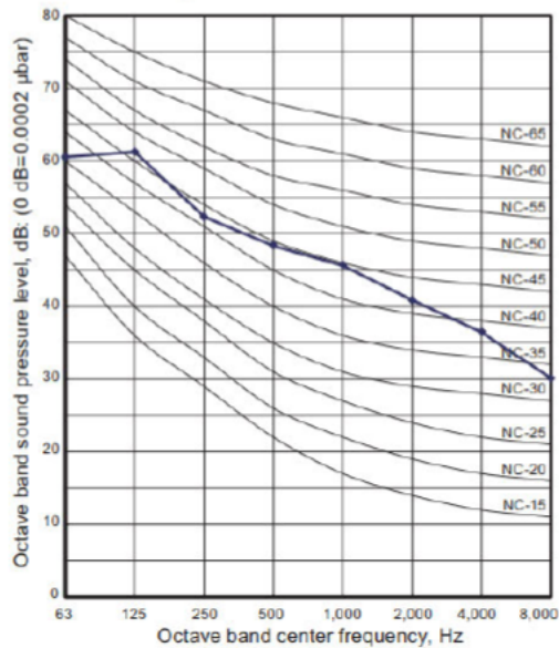
Figure 6.3.2 – Noise Data – Proposed Condenser – 109 Winchester Rd.
