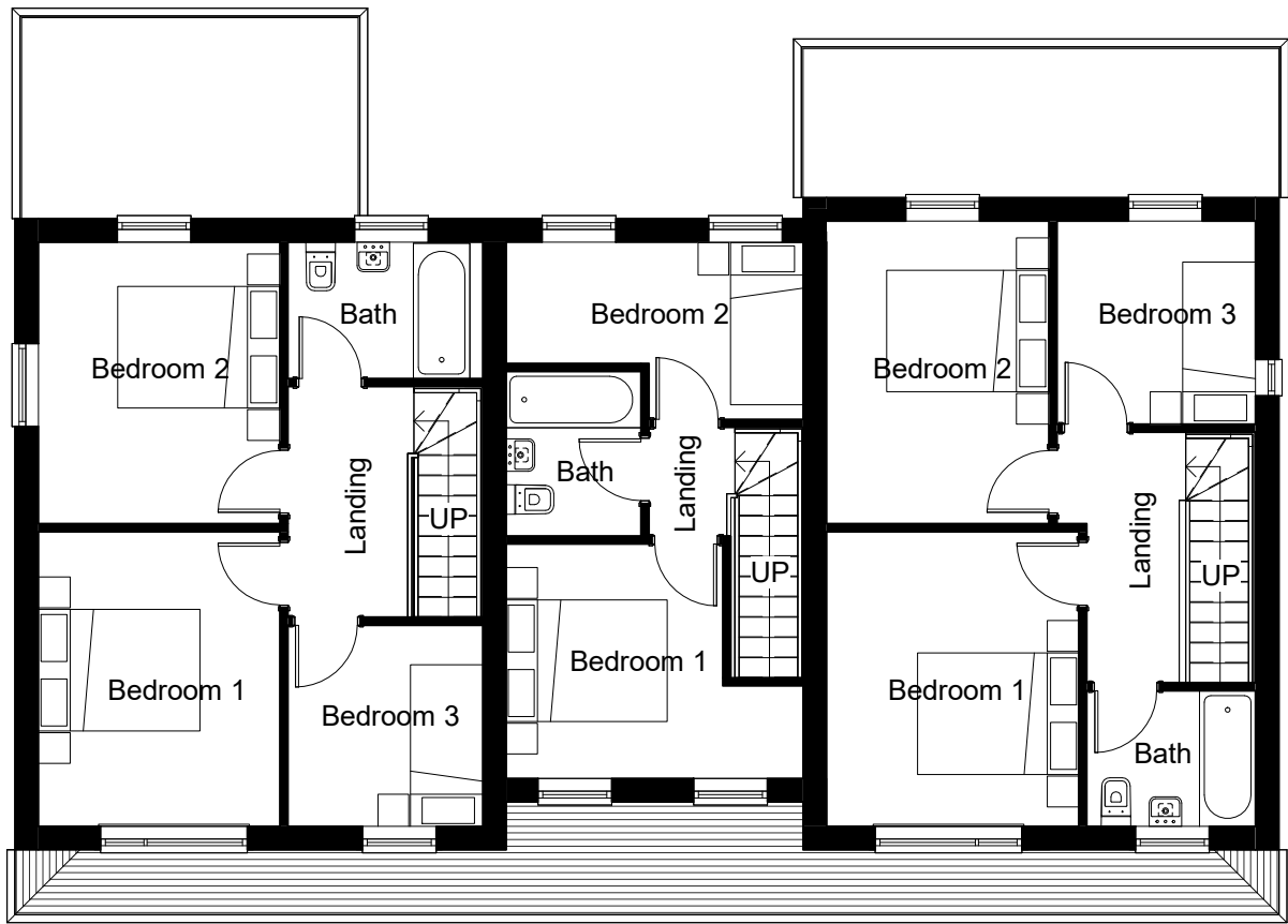
First Floor 1 : 100
