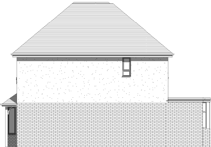
Side Elevation 1 1 : 100
