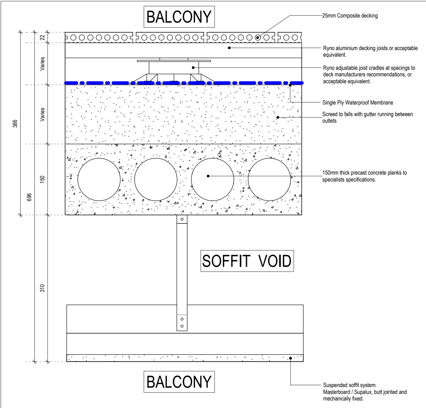
AF13_386_Planks Composite Decking
