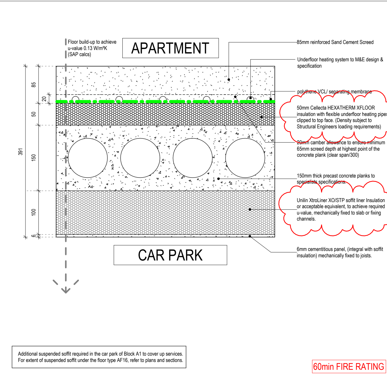
AF16_391_Insulation Planks Screed
