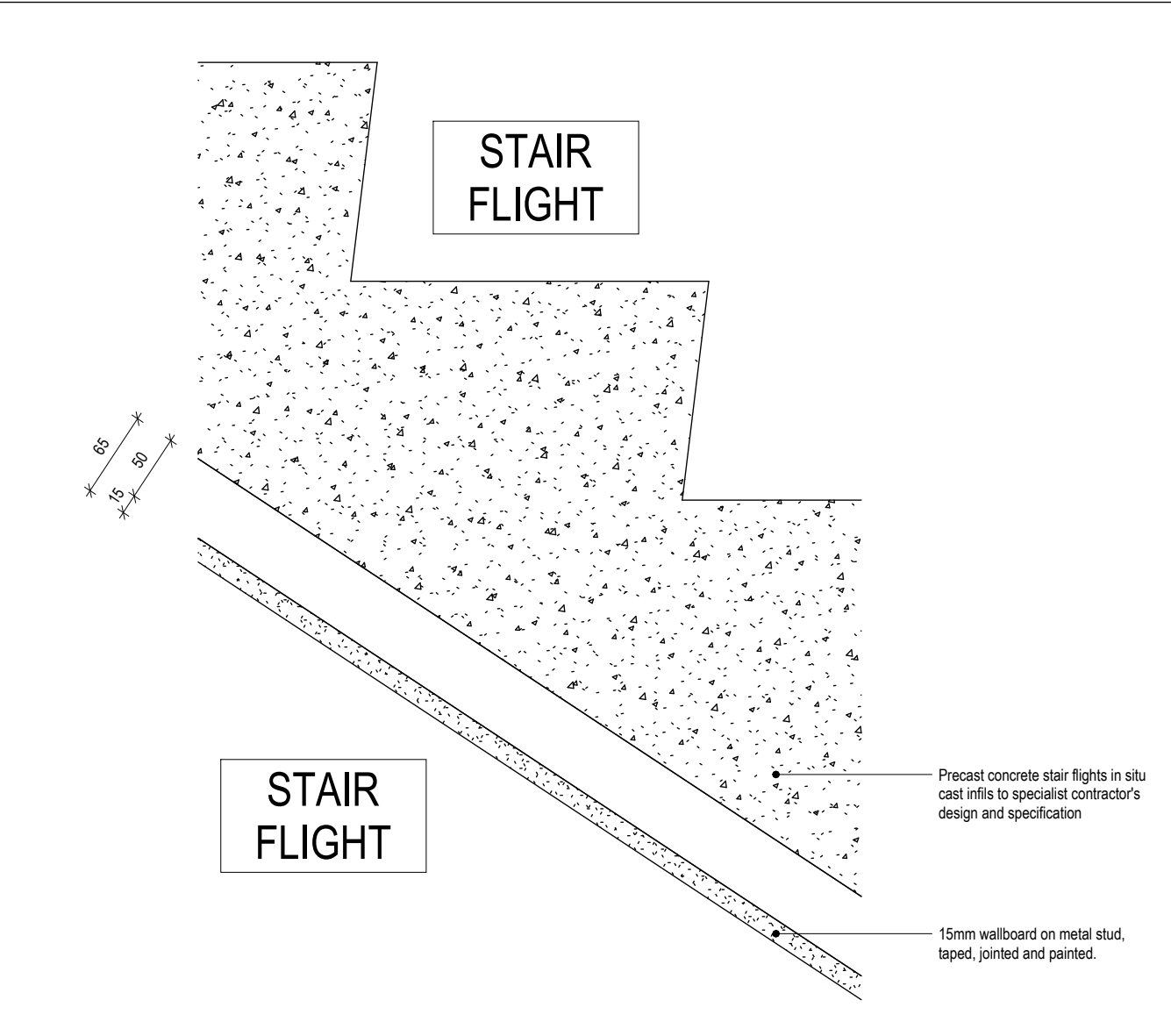
AF19 - Ceiling under stair flight (precast concrete)
