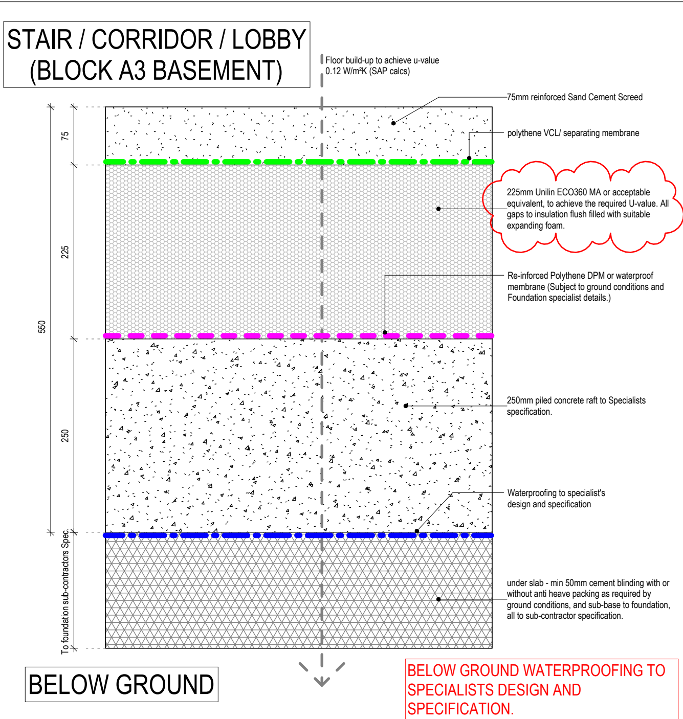
AF23_550_Concrete Insulation Screed
