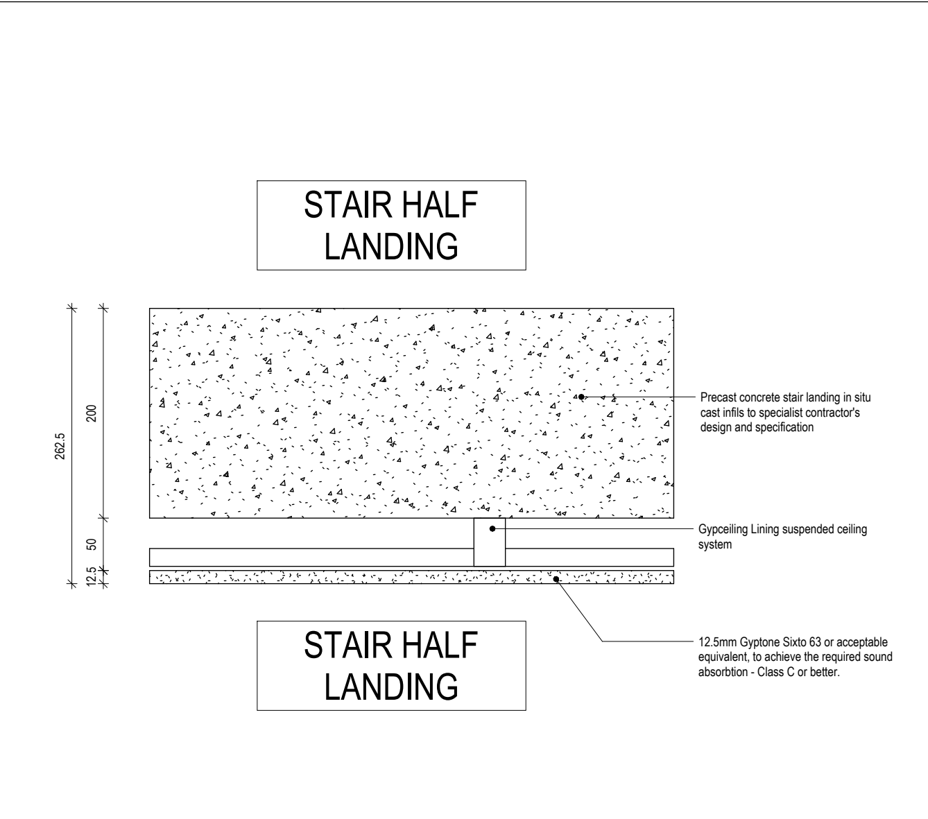
AF20 - Ceiling under half landing
