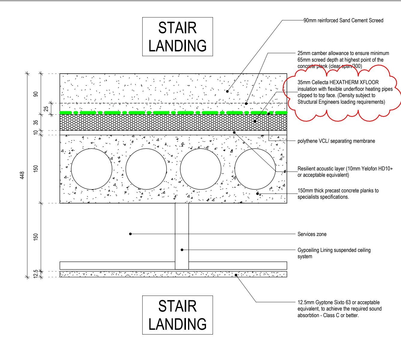
AF18 - Ceiling under stair landing
