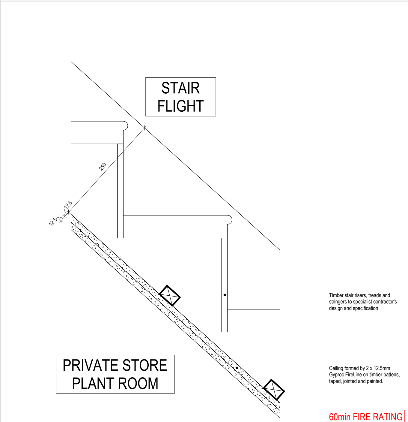
AF22 - Ceiling under stair flight (timber)
