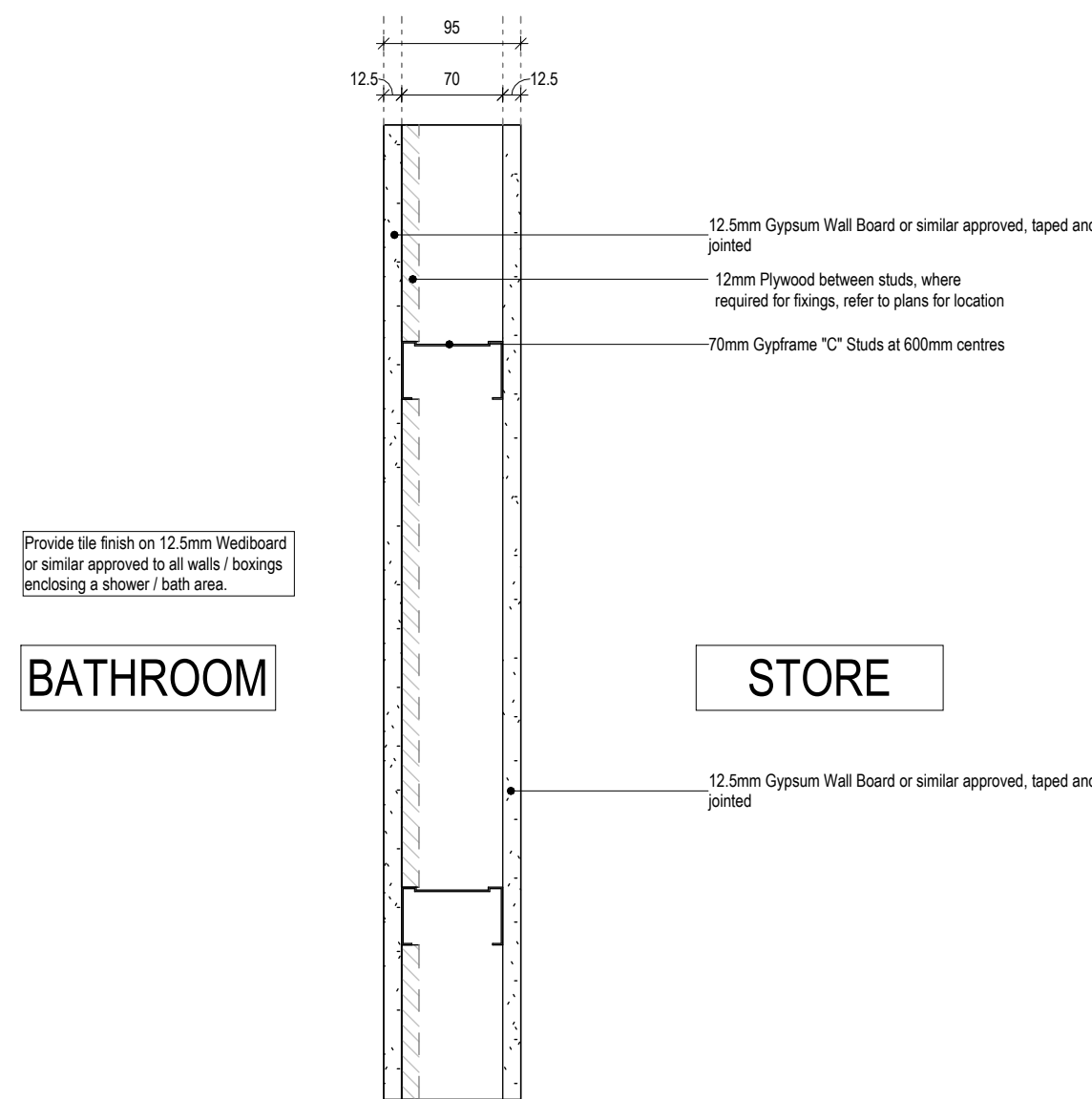
AC4_95_Stud_2x Plasterboard_Ply Pattressing
