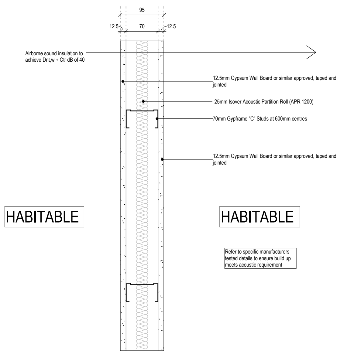
AC2_95_Stud_2x Plasterboard_Acoustic_30min FR
