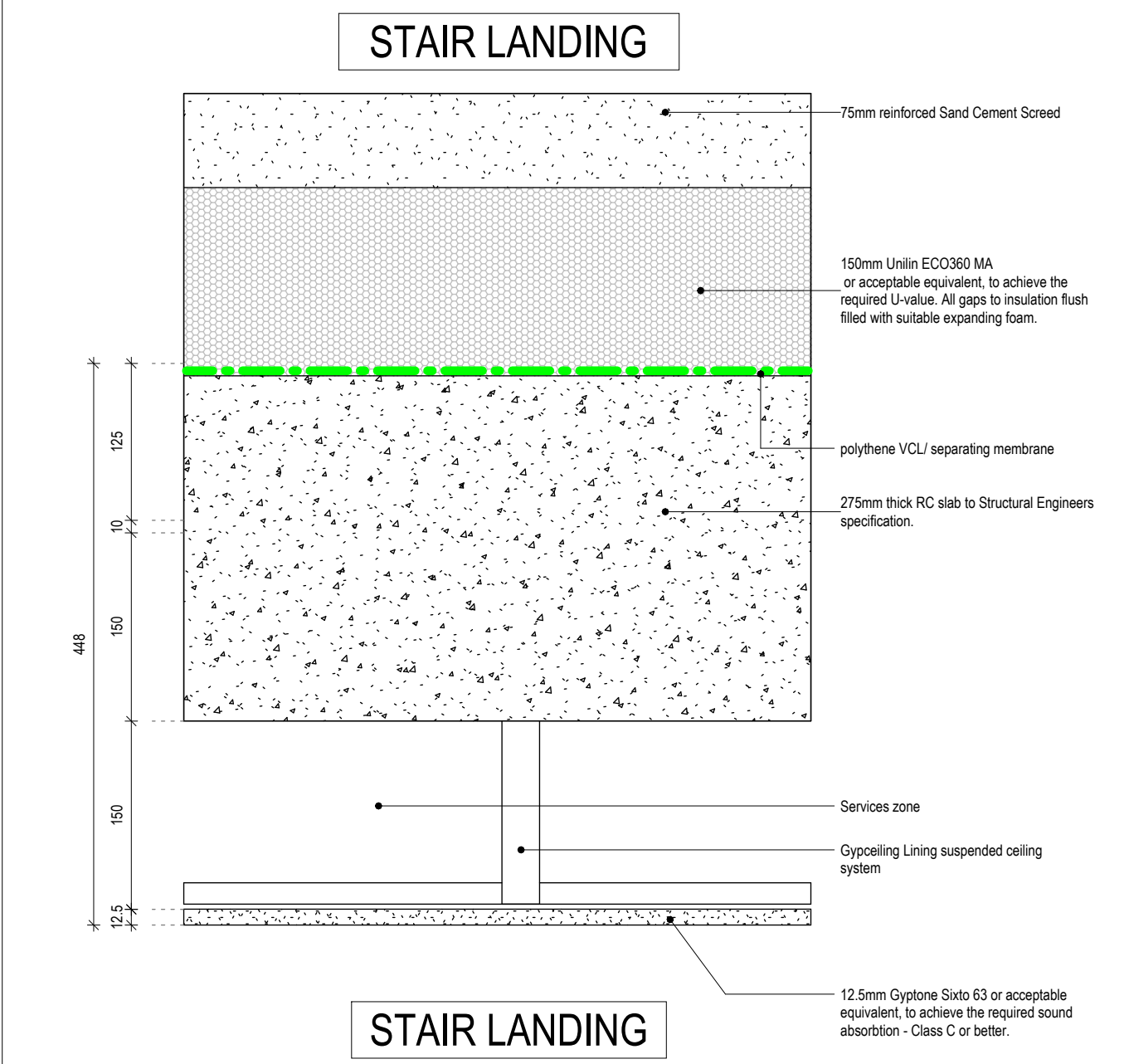
AF26 - Ceiling under stair landing
