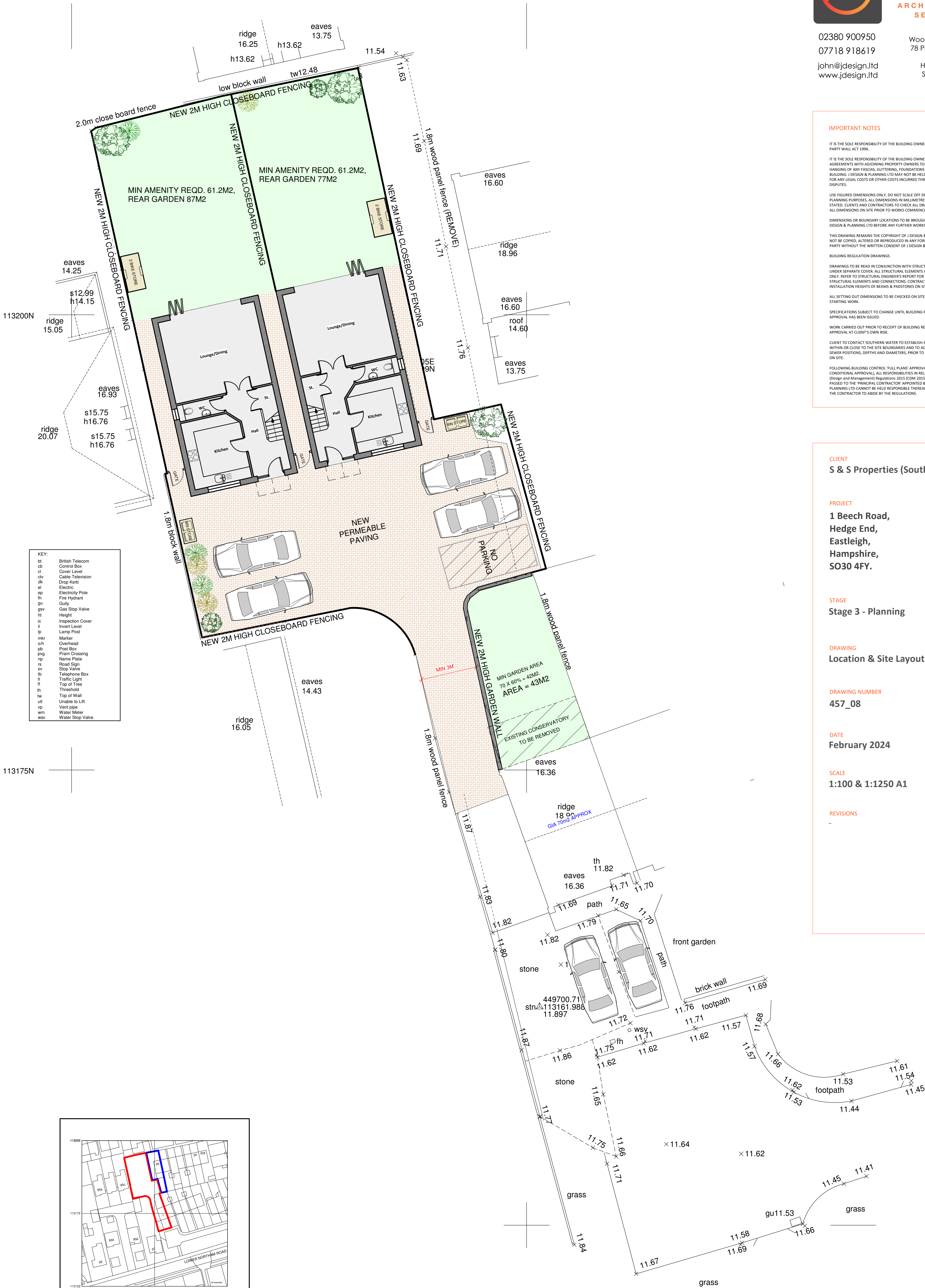
Location Plan 1:1250
