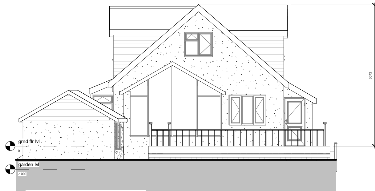
Existing Elevation-Rear
