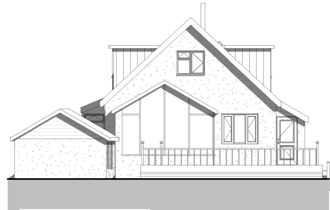
Proposed Elevation-Rear
