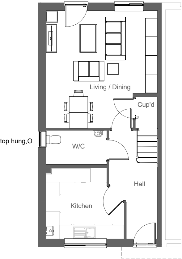
Ground Floor Plan O= Obscure glazed window.
