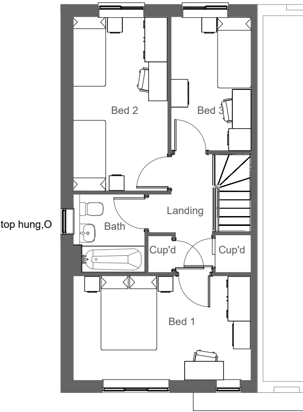
First Floor Plan O= Obscure glazed window.
