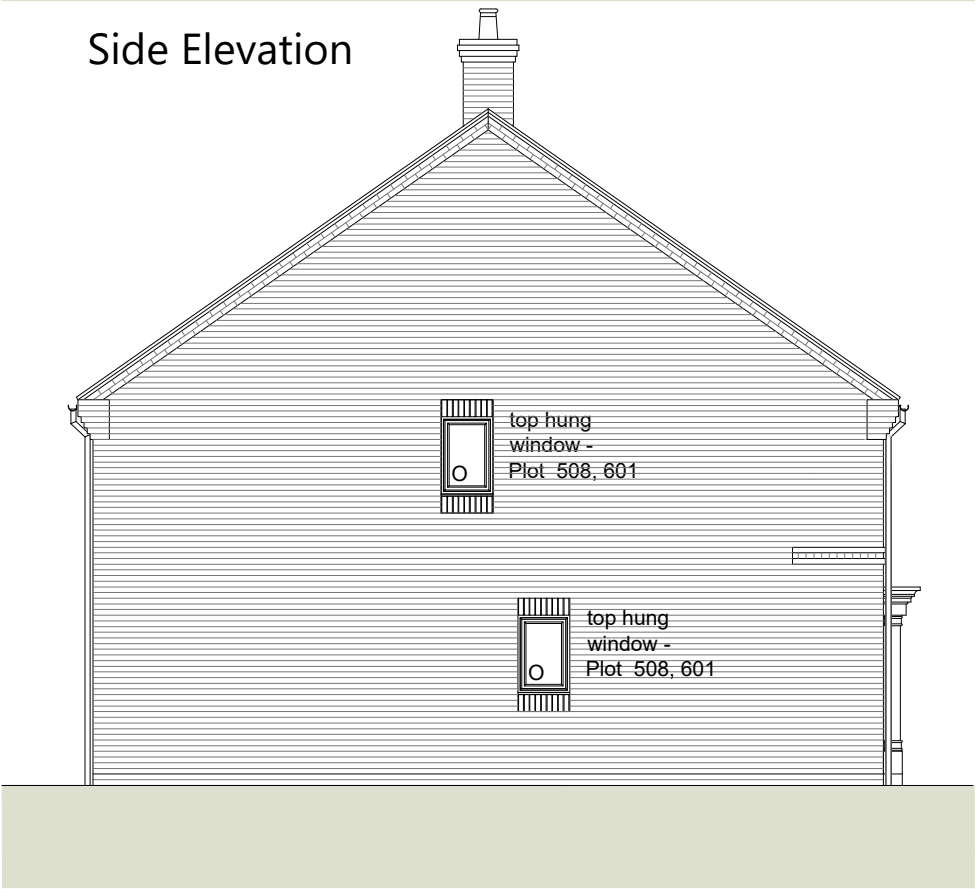
Side Elevation O= Obscure glazed window.
