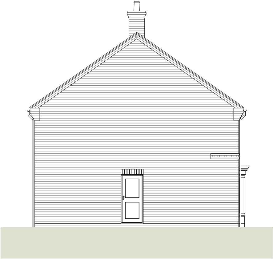
Side Elevation
