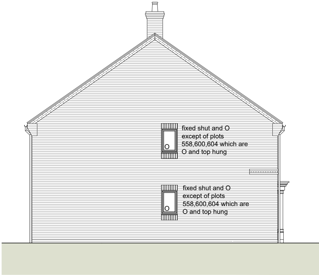
Side Elevation
