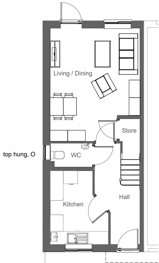
Ground Floor Plan O= Obscure glazed window.
