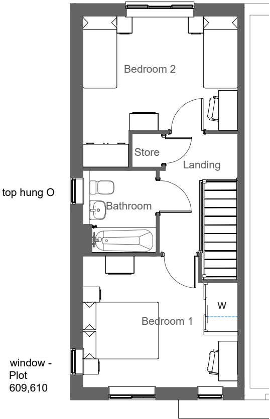
First Floor Plan O= Obscure glazed window.
