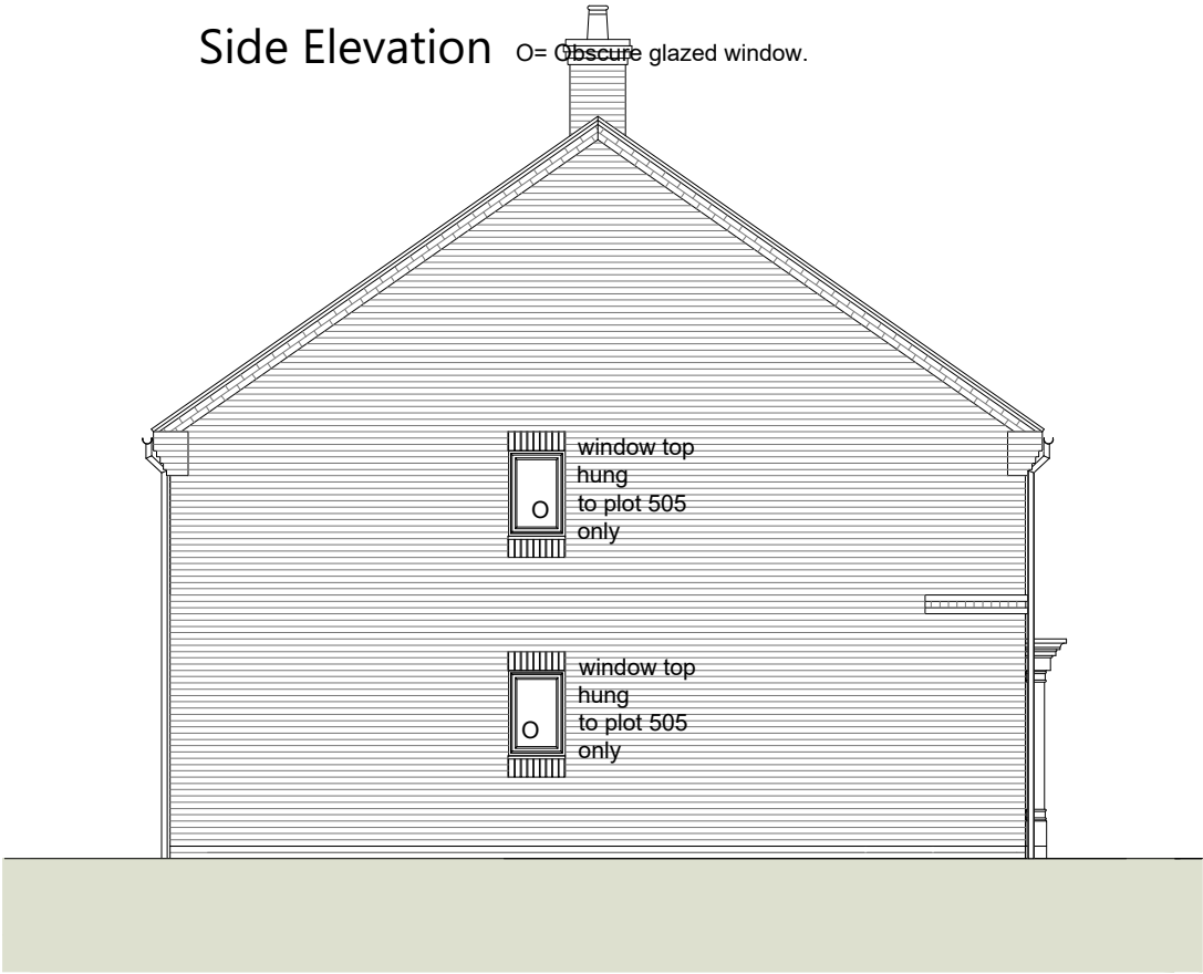
Side Elevation O= Obscure glazed window.
