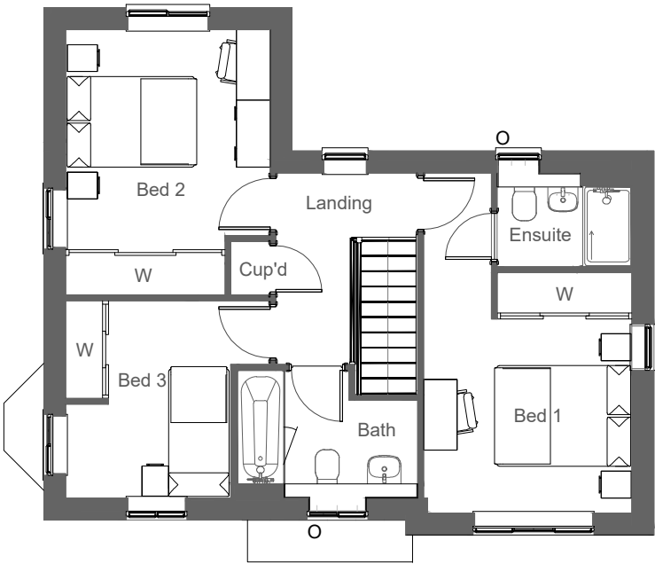
First Floor Plan O= Obscure glazed window.
