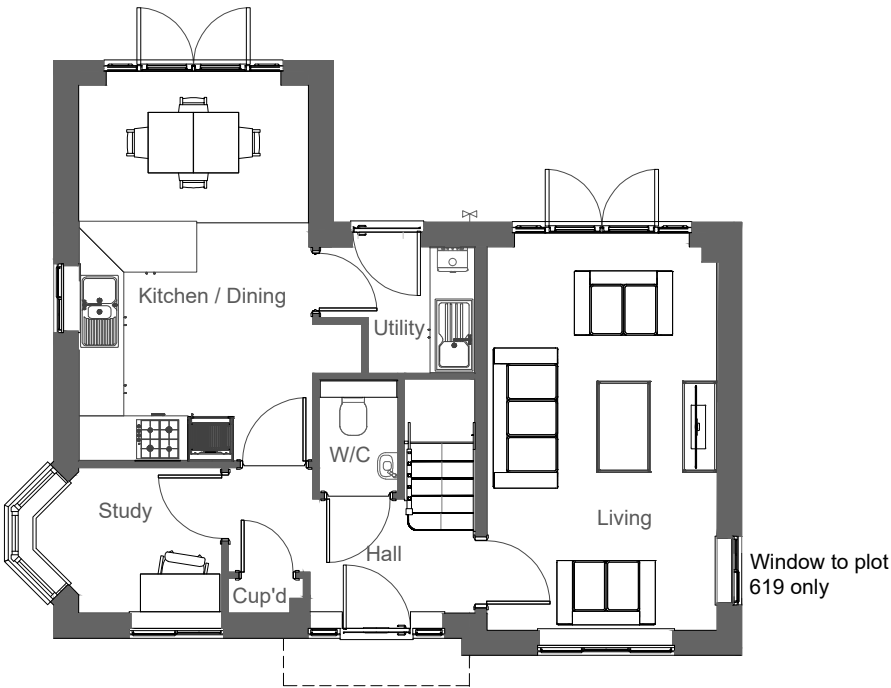
Ground Floor Plan O= Obscure glazed window.
