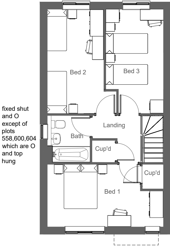
First Floor Plan O= Obscure glazed window.
