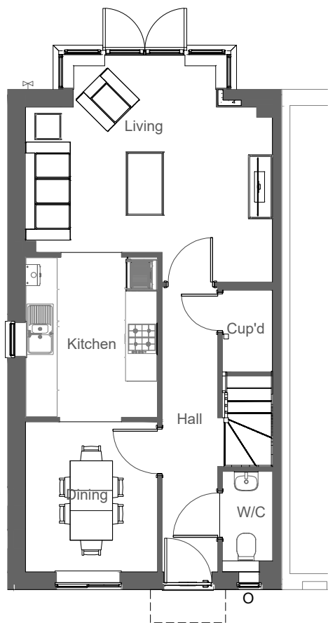
Ground Floor Plan O= Obscure glazed window.
