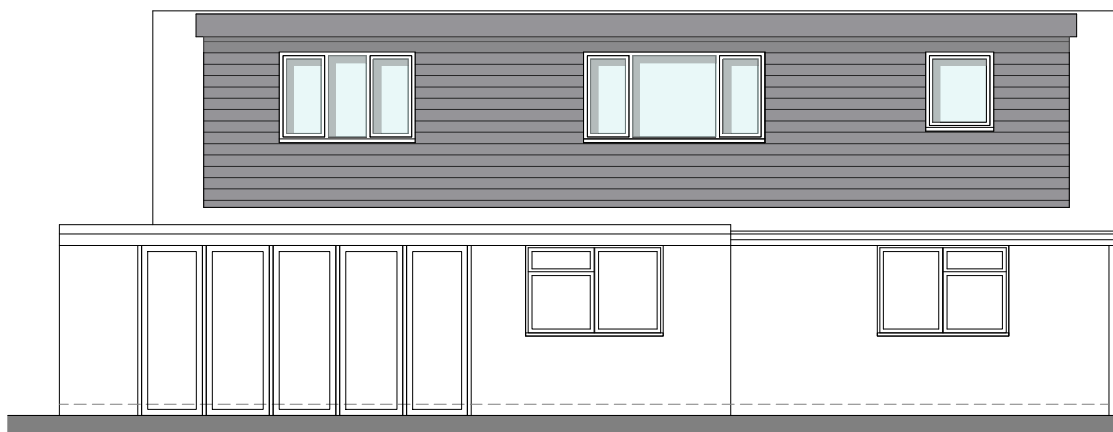
REAR ELEVATION
