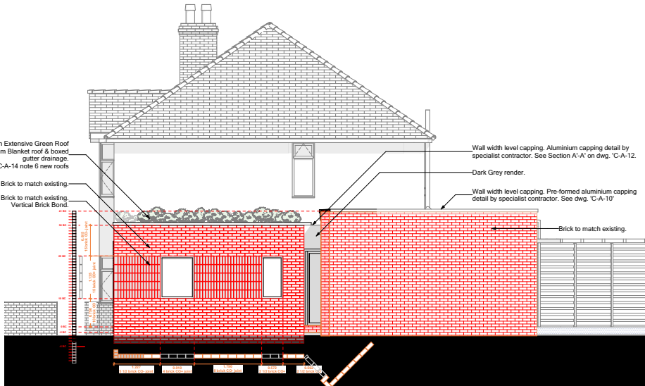
3 Side Elevation - PROPOSED 1:50
