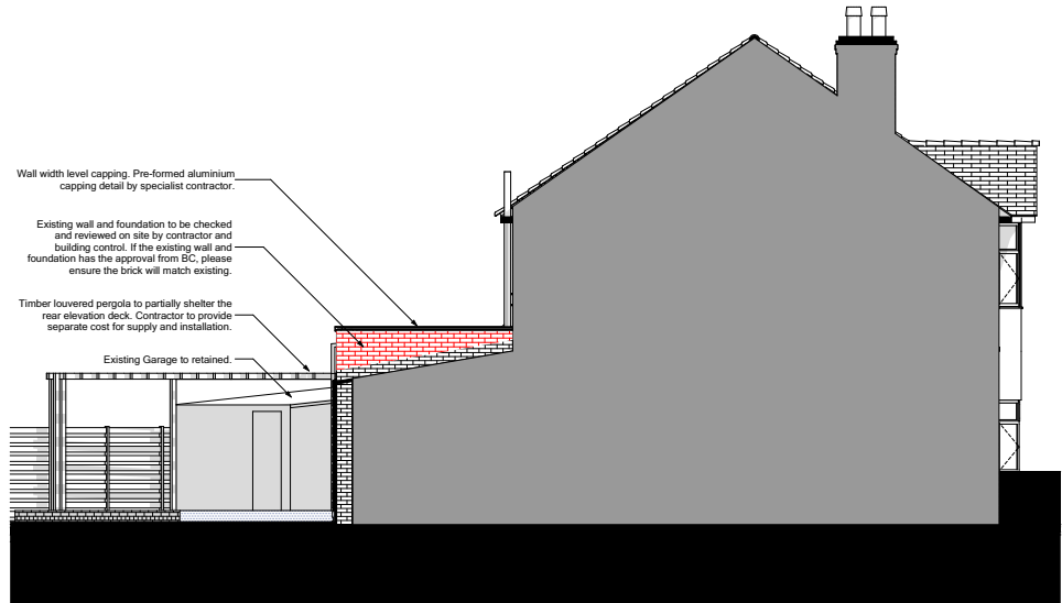
4 Side Elevation - PROPOSED 1:50
