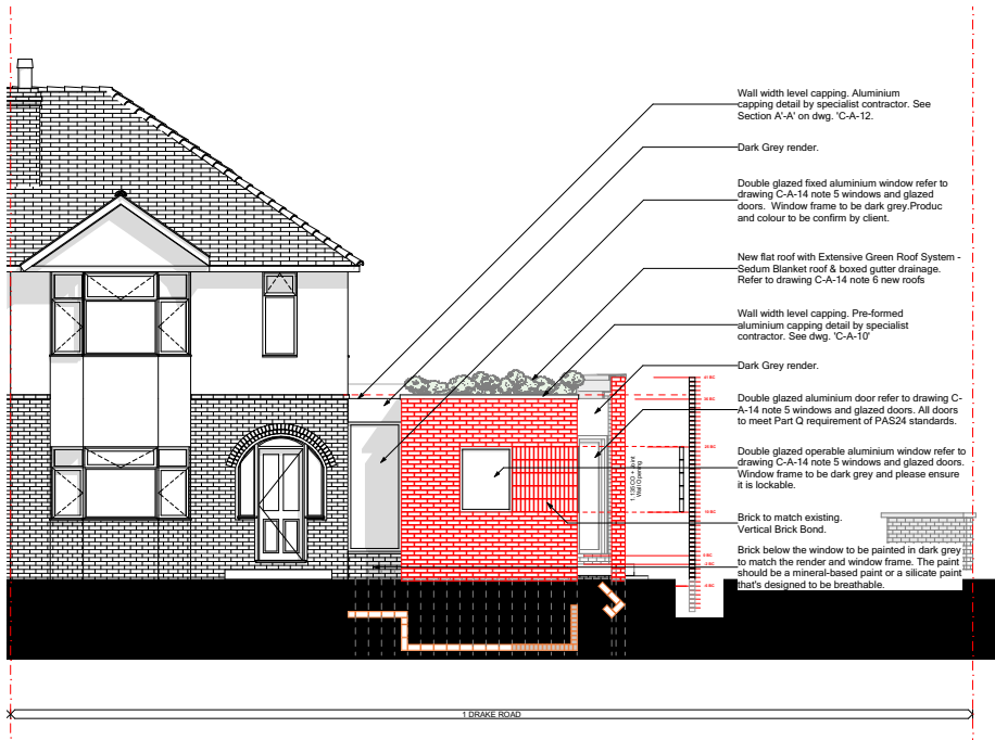
1 Front Elevation - PROPOSED 1:50
