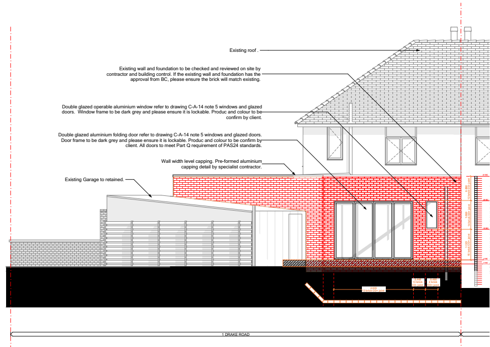
2 Rear Elevation - PROPOSED 1:50
