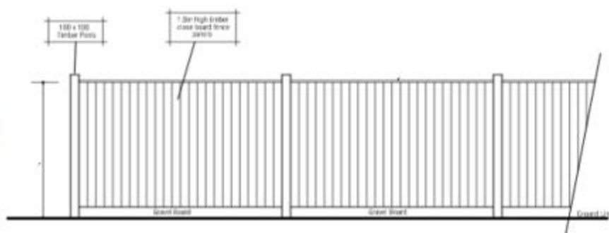
Section 1 Fence - 2 metre length, Left to Right from bungalow
