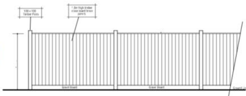
Section 2 Fence - 2 metre length, dropped height from Section 1
