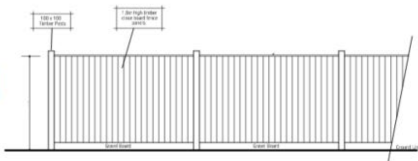
Section 3 Fence – 19 metre length, inside ground level enclosing lower garden area
