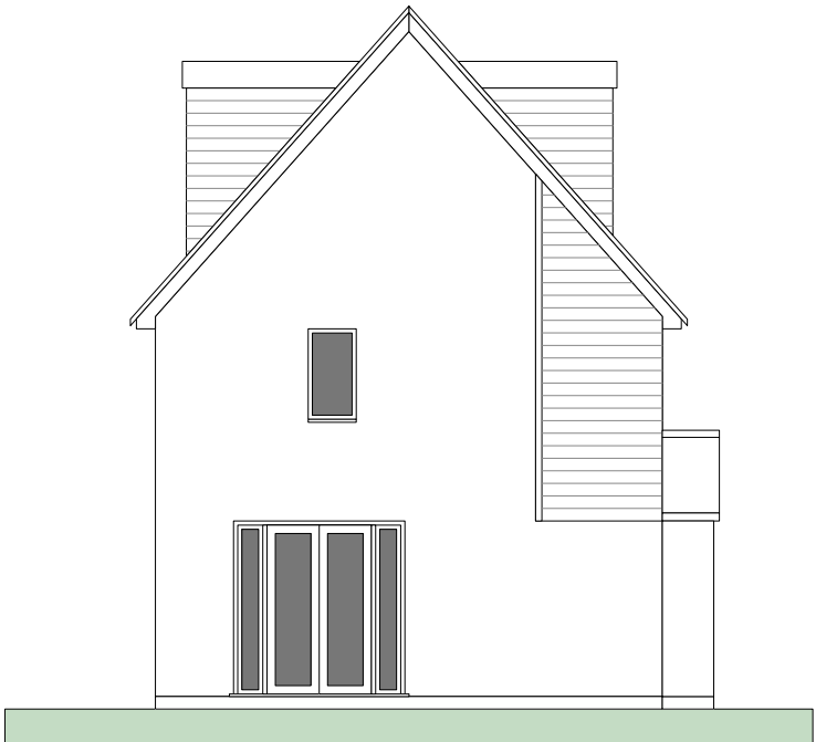
NORTH ELEVATION
