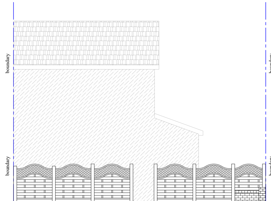
Proposed West Elevation 1:100 @A3
