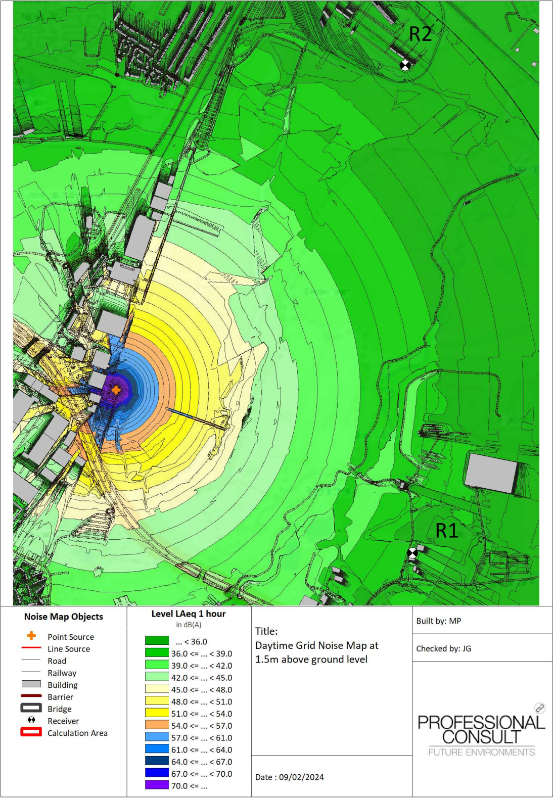
Figure 2 – Daytime Grid Noise Map – Phase 1
