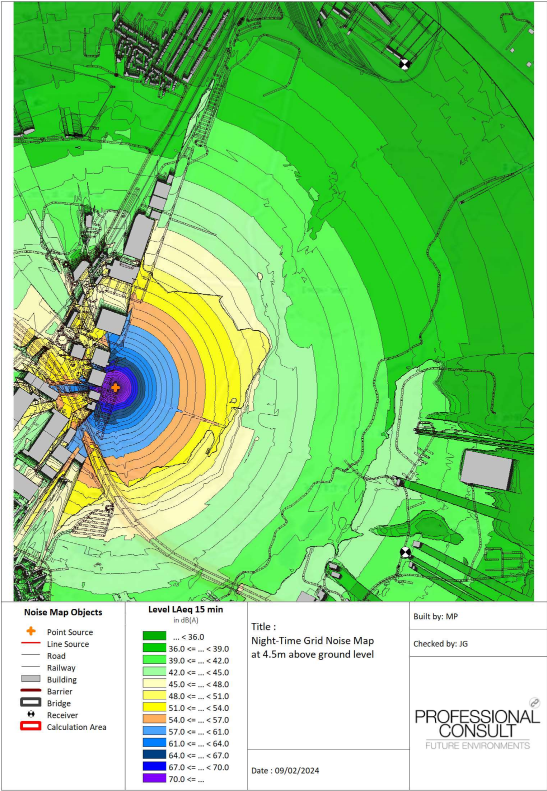
Figure 3 – Night-Time Grid Noise Map
