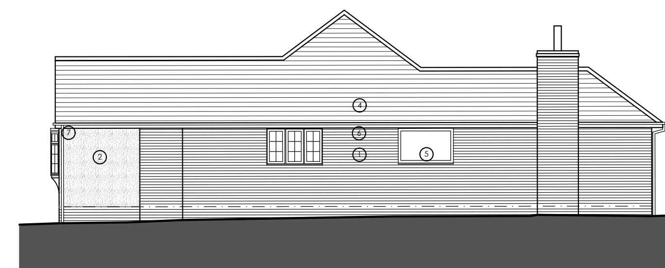
50.0m DATUM SIDE, NORTH ELEVATION
