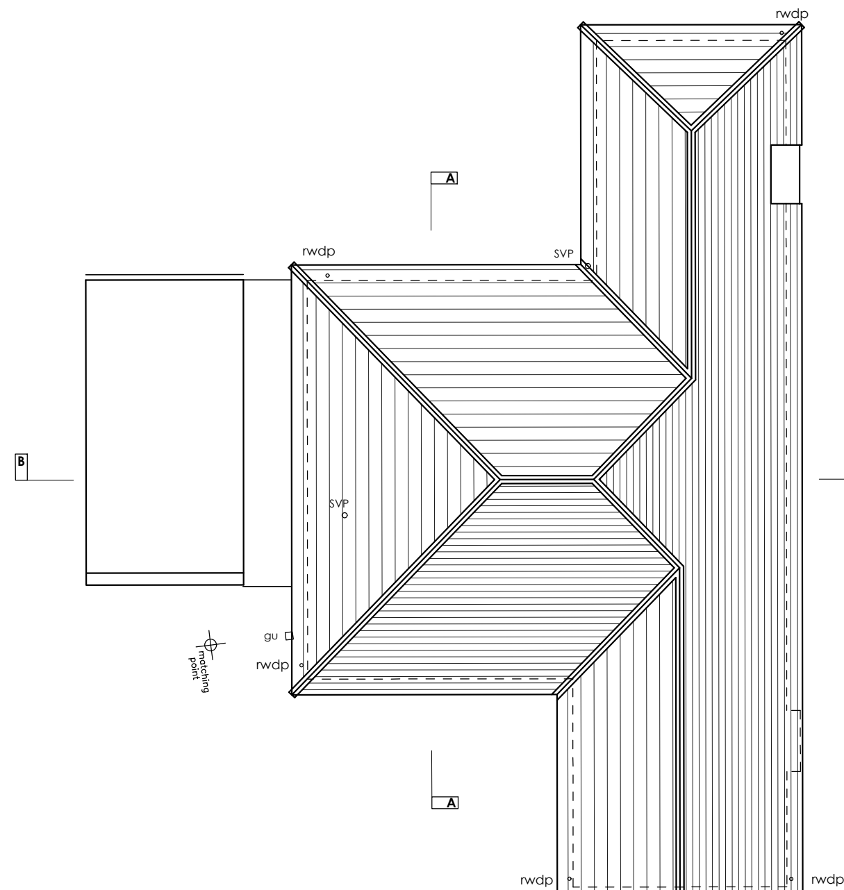
ROOF PLAN
