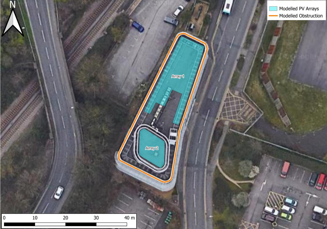
Figure 5.3 Modelled Obstruction
