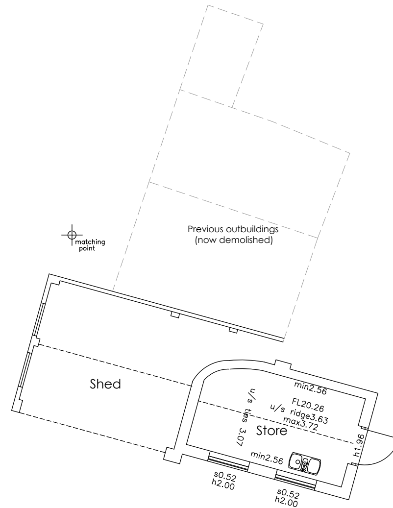
OUTBUILDING FLOOR PLAN
