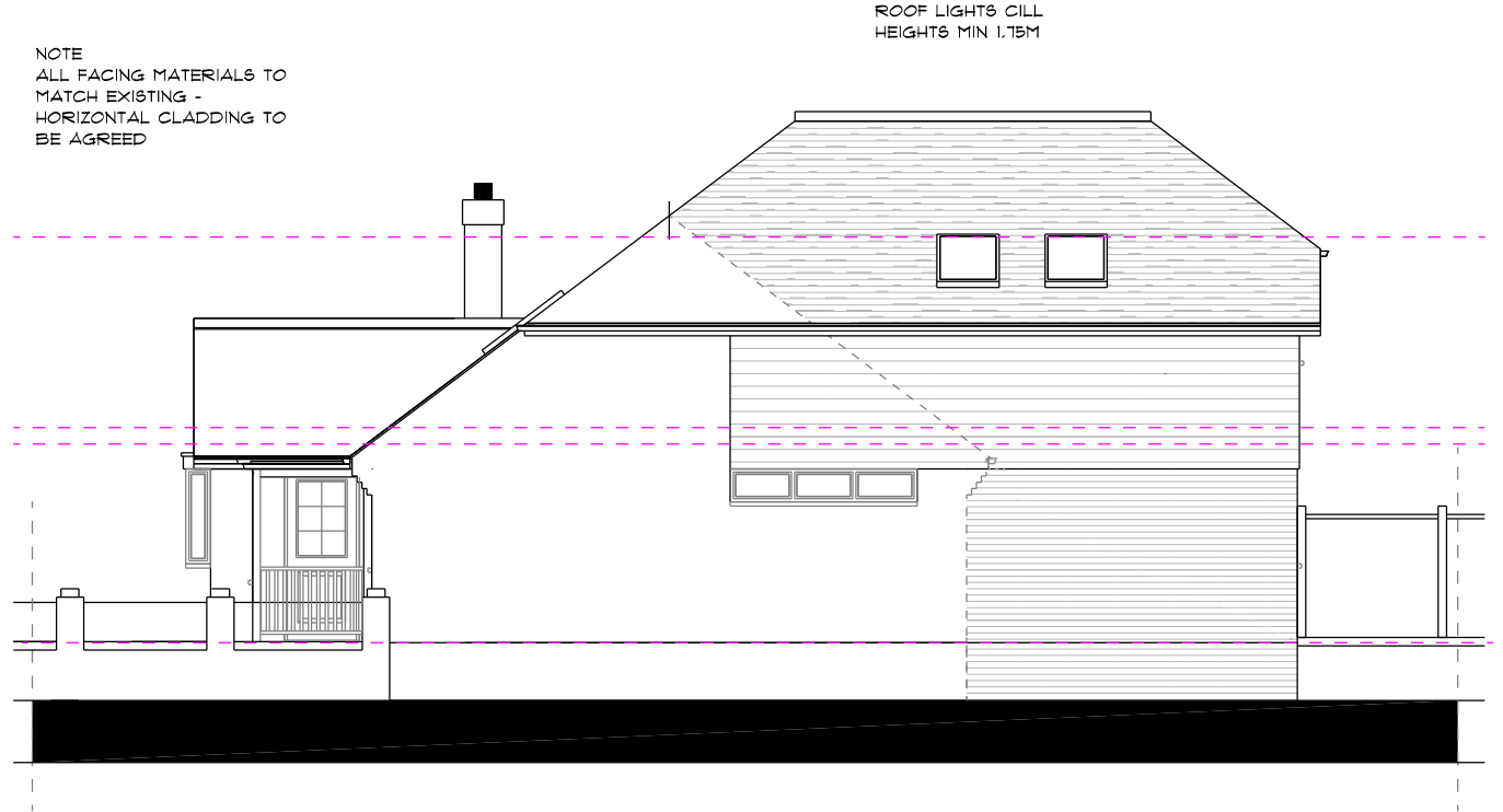
PROPOSED EAST ELEVATION - SIDE Scale 1:100 @ A3
