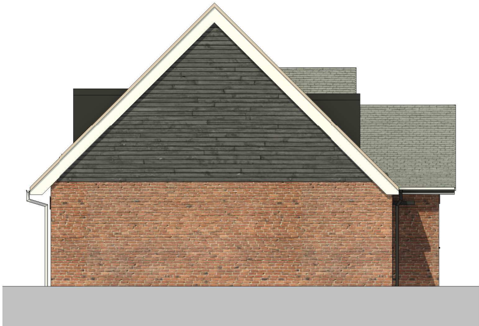
③ North West Elevation 1 : 100
