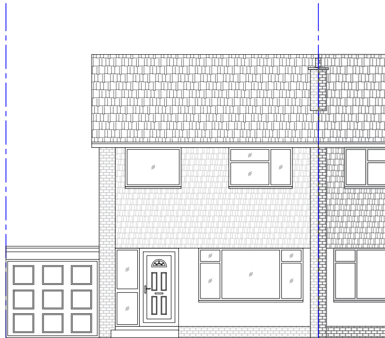
Existing Front Elevation 1:100 @A3
