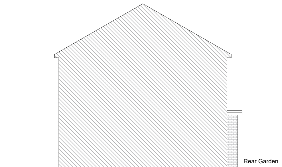
Proposed East Elevation 1:100 @A3
