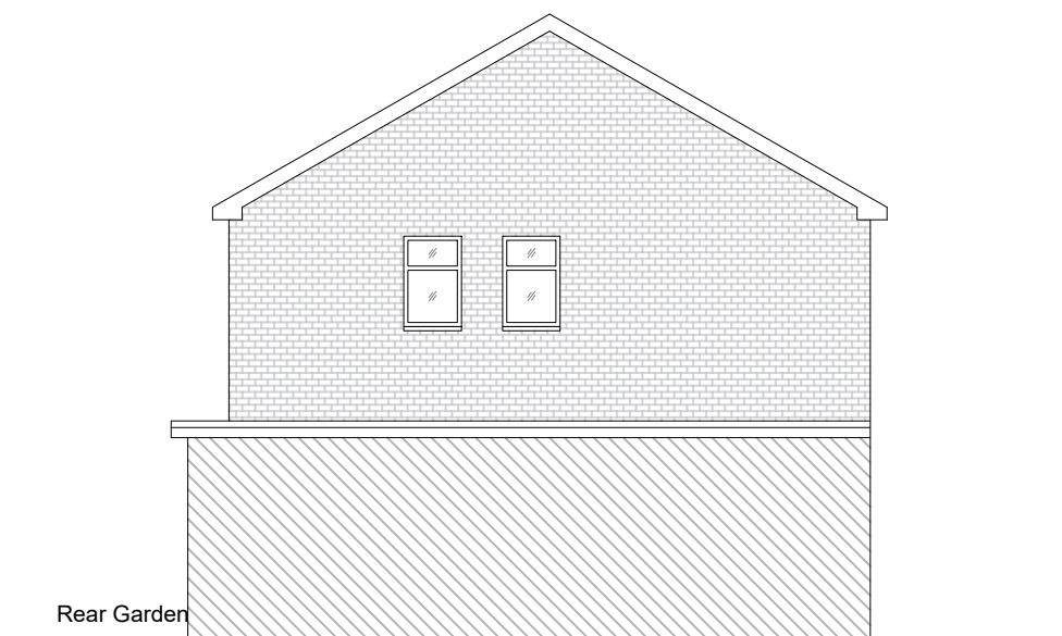
Proposed West Elevation 1:100 @A3
