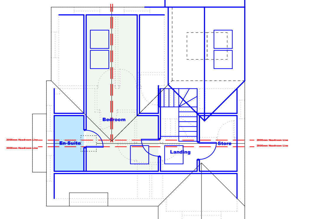
Proposed Second Floor Plan 1:100
