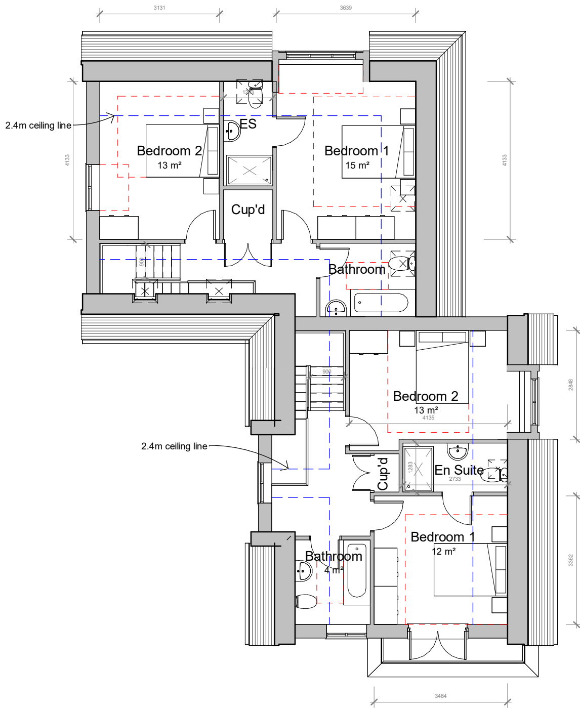
2 1 First Floor FFL 1 : 100
