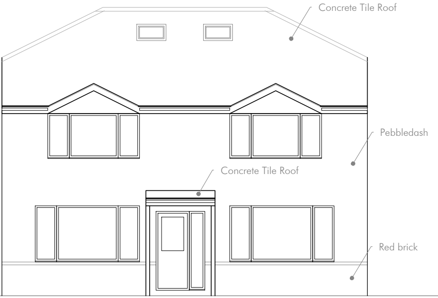
Existing Front / East Elevation
