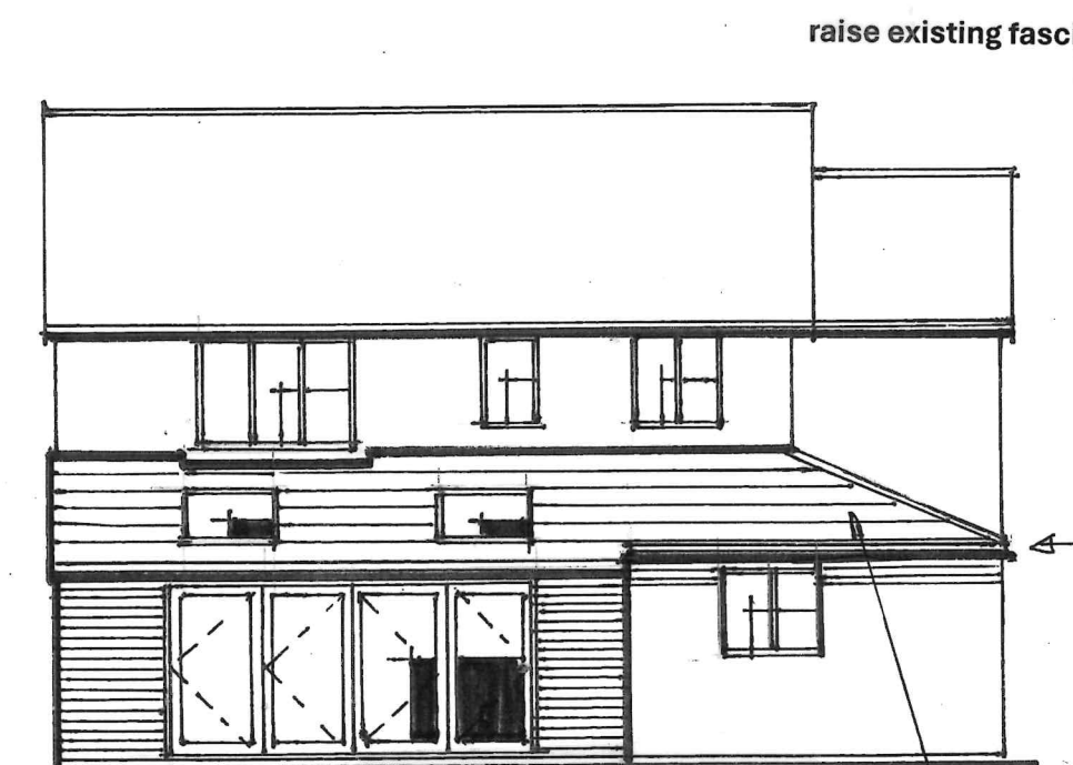
REAR ELEVATION - PROPOSED
