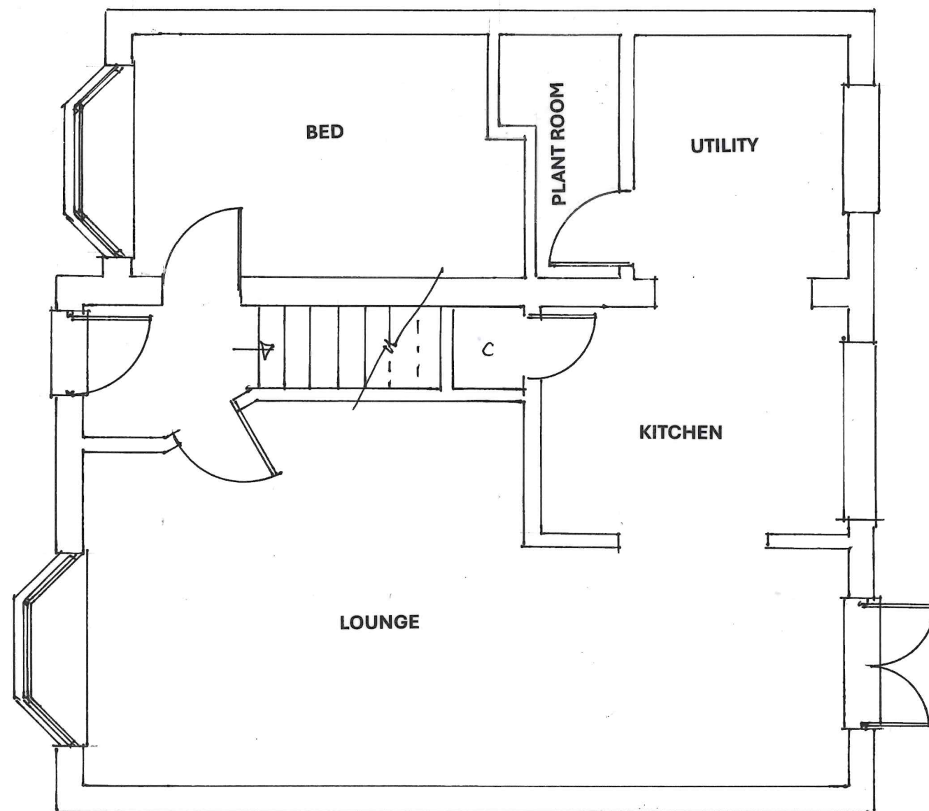
GROUND FLOOR - EXISTING
