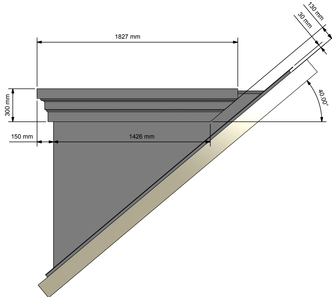
Side Elevation ( 1:20 )
