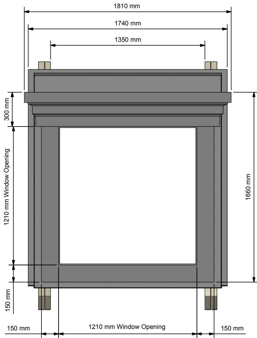
Front Elevation ( 1:20 )
