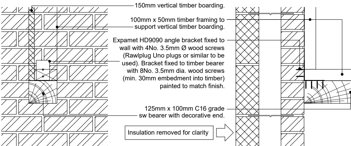
D5 - SECTION DETAIL OF BRACKET / BEARER / CONNECTION TO EXTERNAL WALL (scale 1:10)
