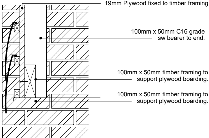
SECTION DETAIL OF BEARER / CONNECTION TO EXTERNAL WALL (scale 1:10)
