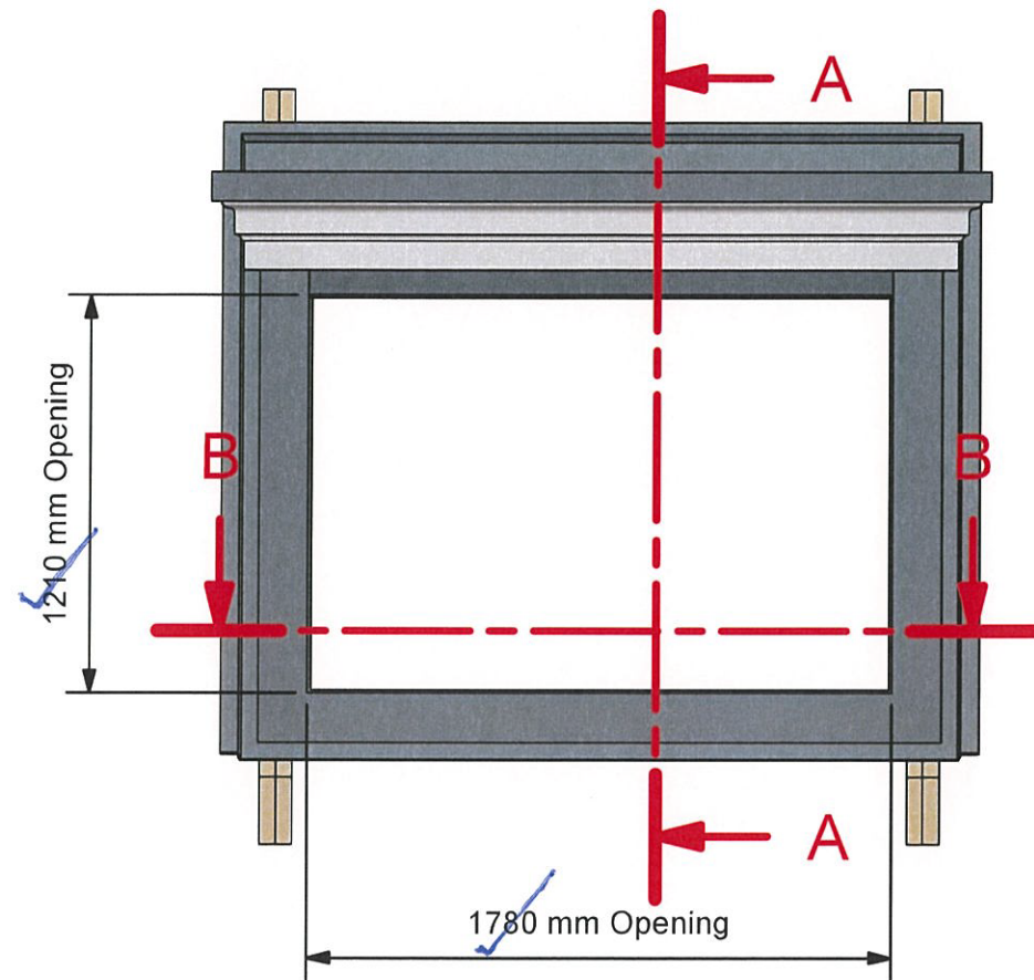
Front Elevation ( 1 : 35 )
