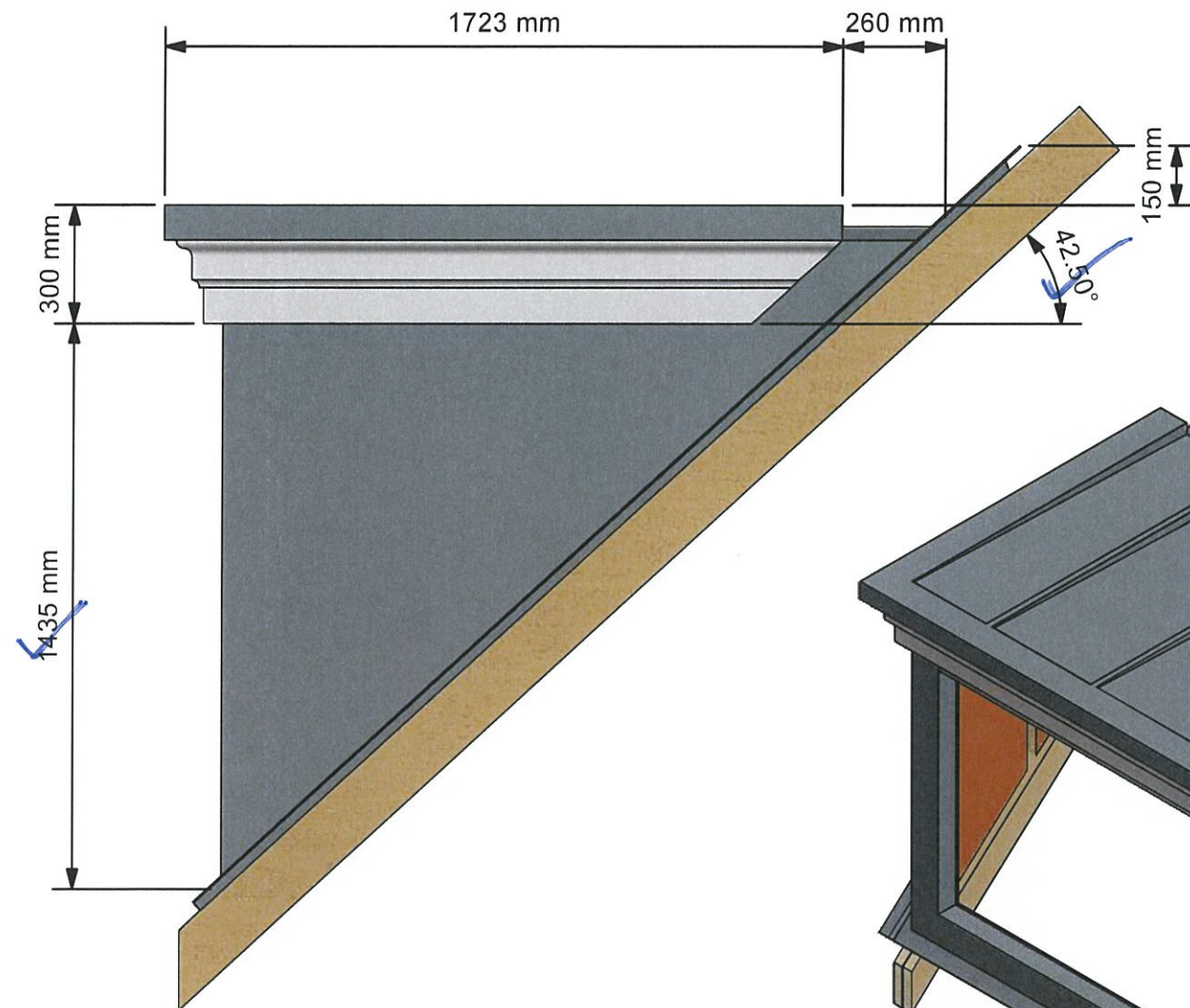
Auxiliary View ( 1 : 40 )
