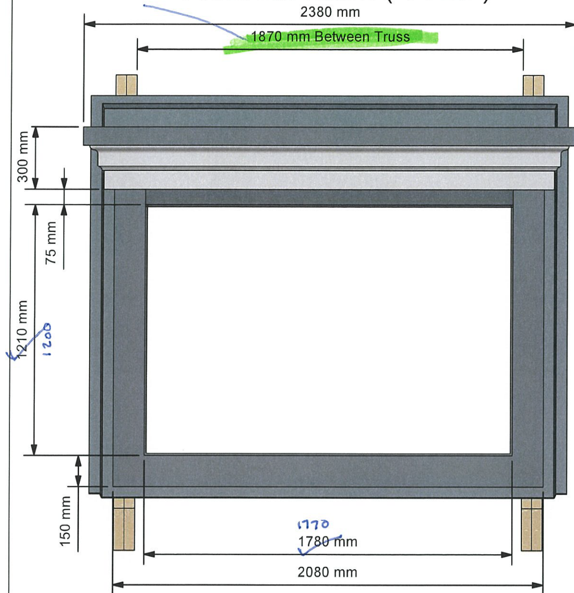
Front Elevation ( 1 : 25 )
