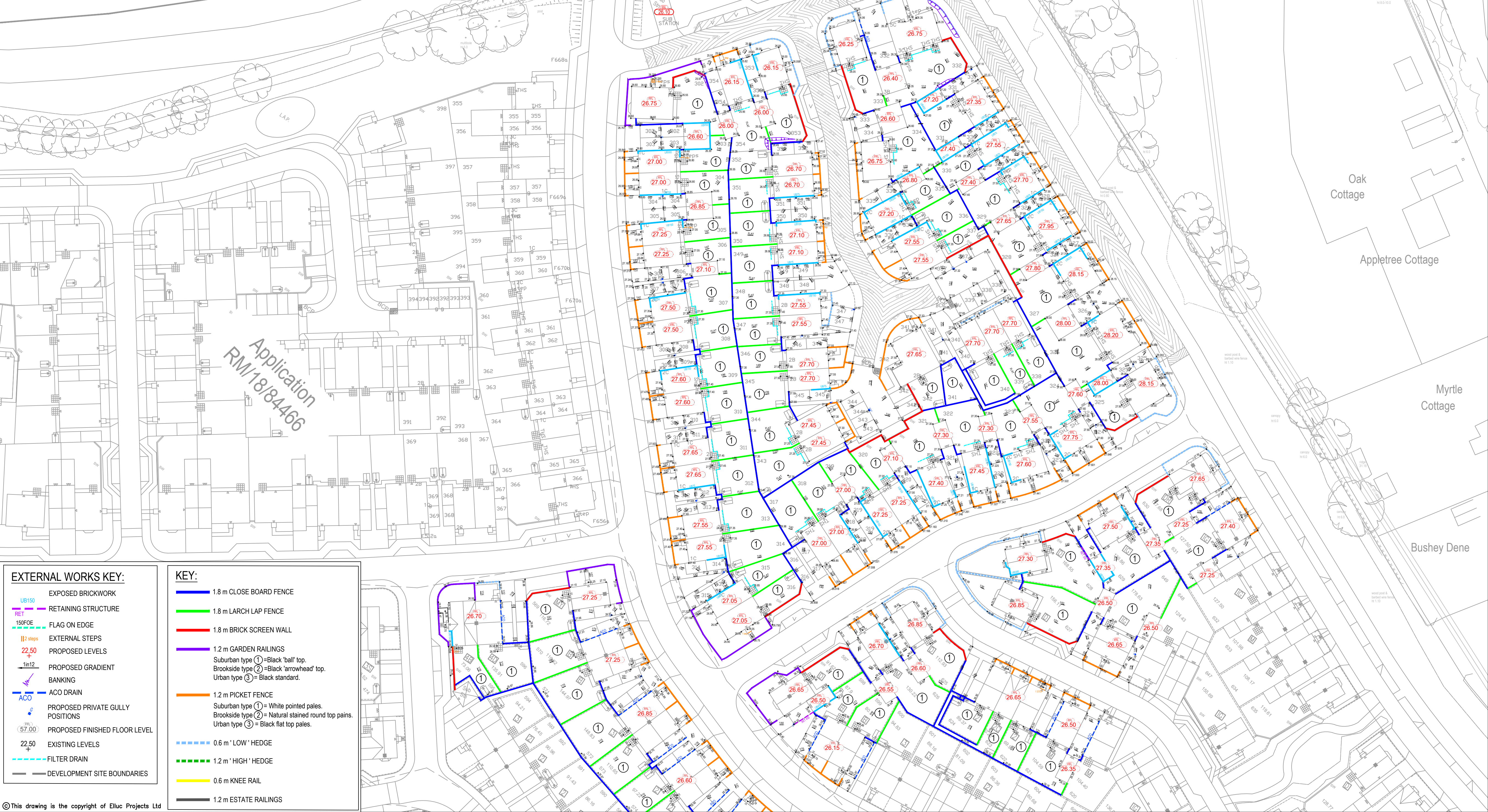
EXTRACT FROM SOUTH WEST OF SITE SCALE - 1:500
