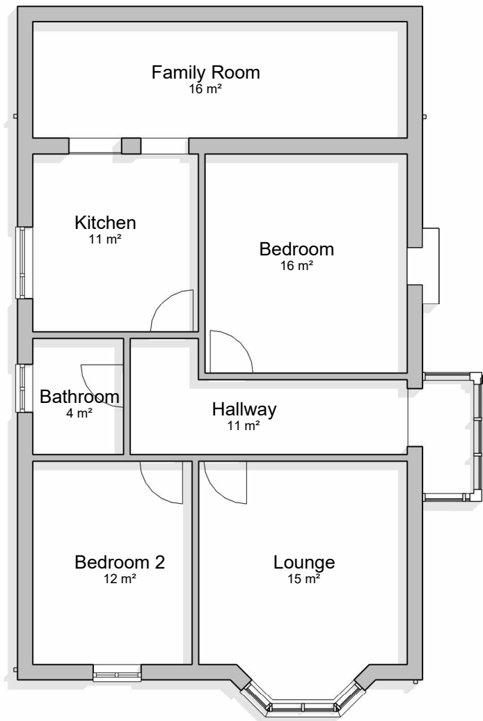
1 Existing Gnd Floor 1 : 100
