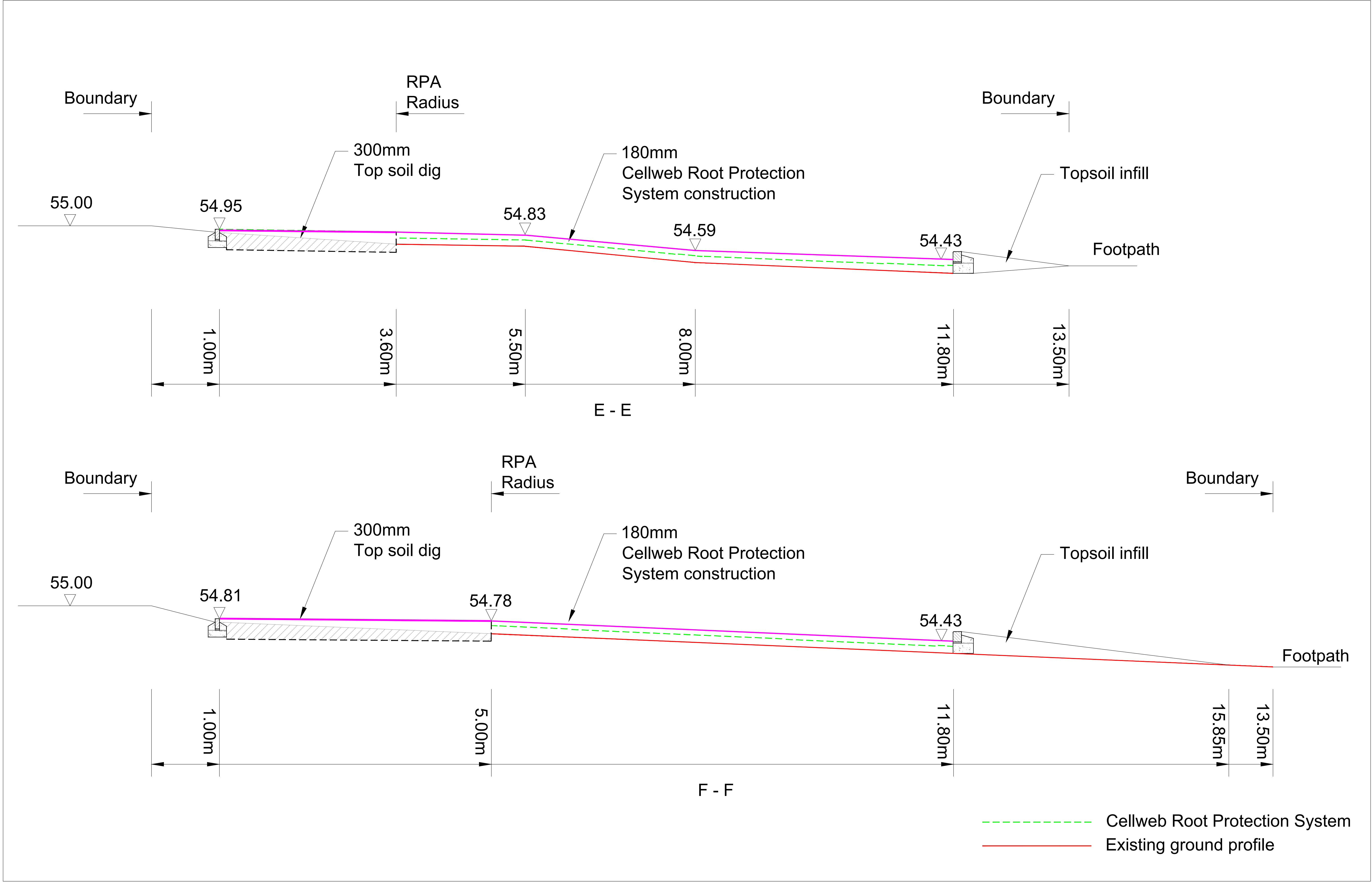
Cross sections E-E and F-F Scale 1:25 @ A1
