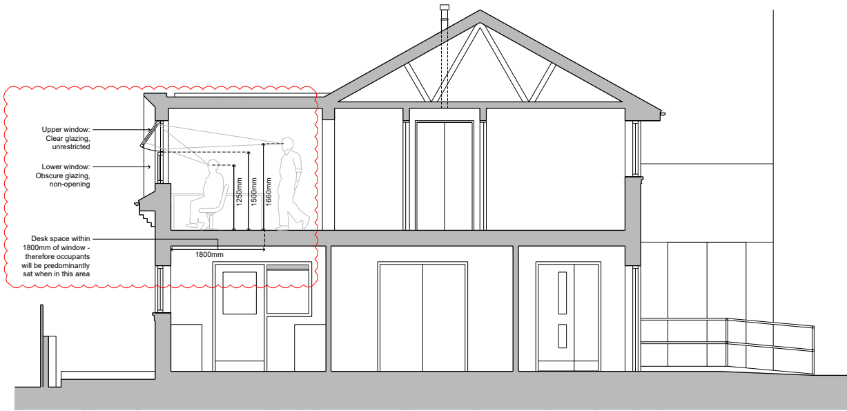
PROPOSED SECTION
