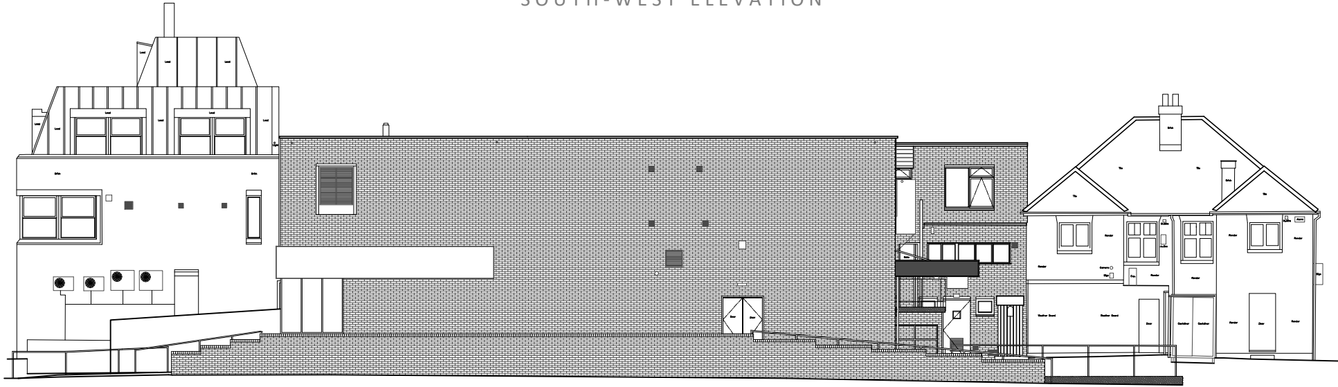
SOUTH-WEST ELEVATION
