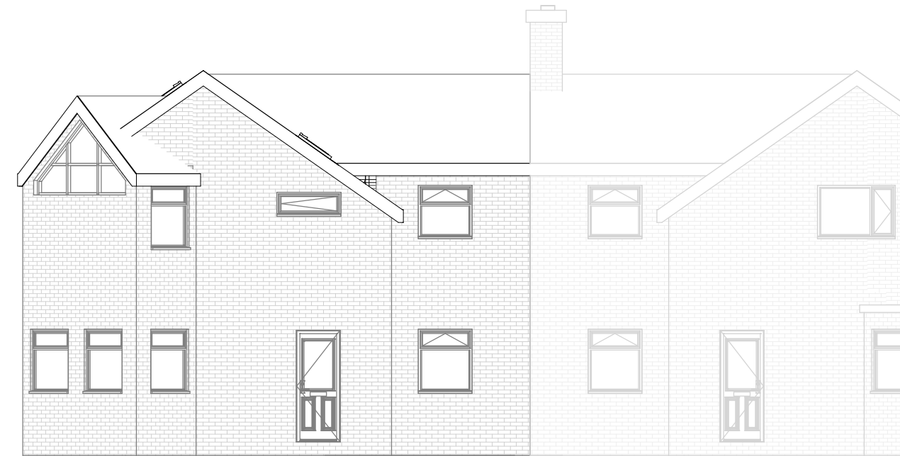
Proposed Elevation-Front
