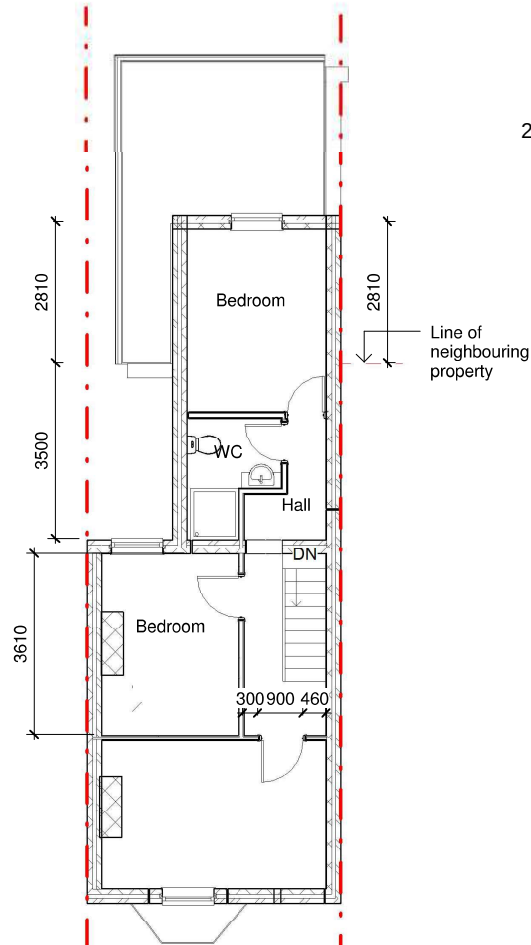
Proposed First Floor Plan NH 1 : 100
