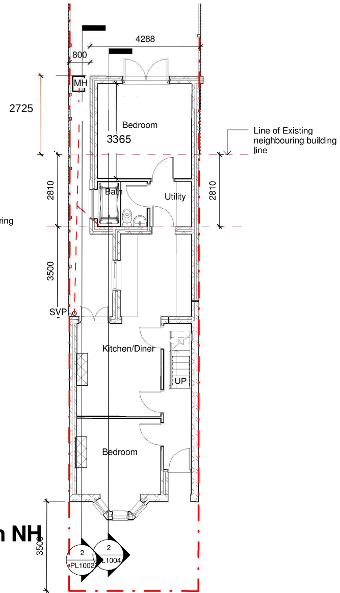
Proposed Ground Floor Plan NH 1 : 100
