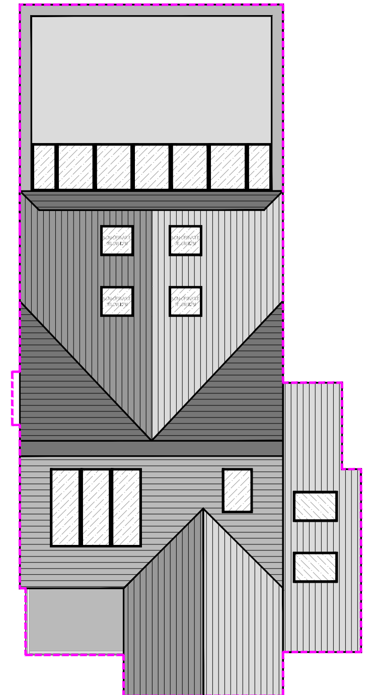
ROOF | PROPOSED
