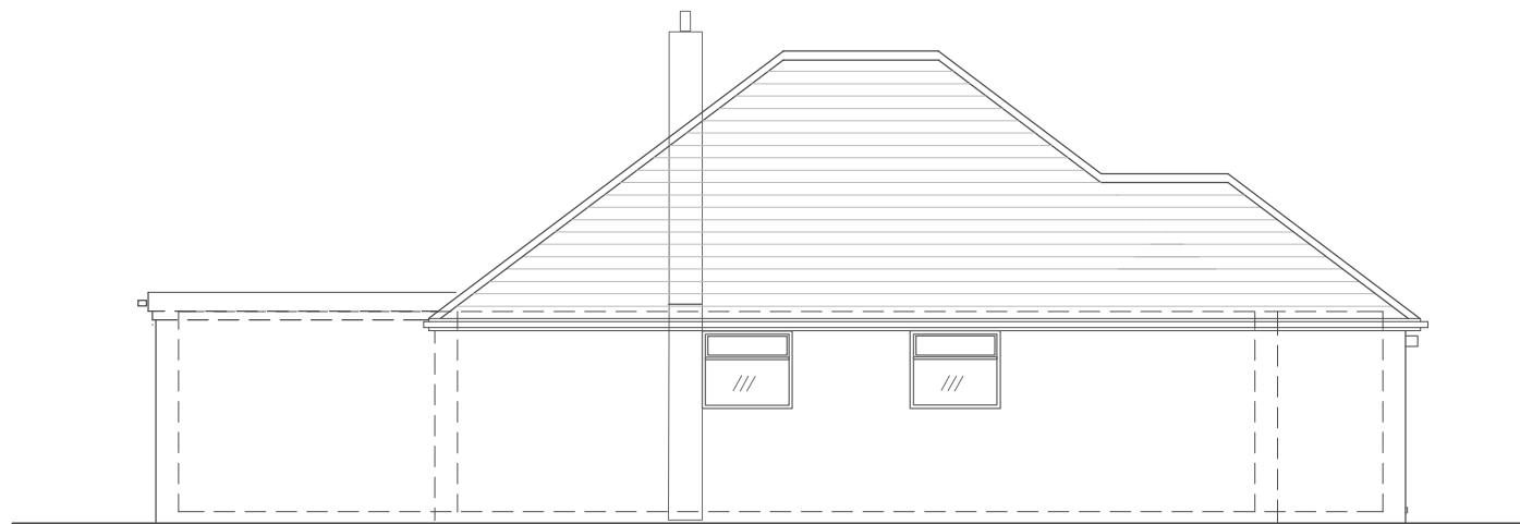
SouthElevation
